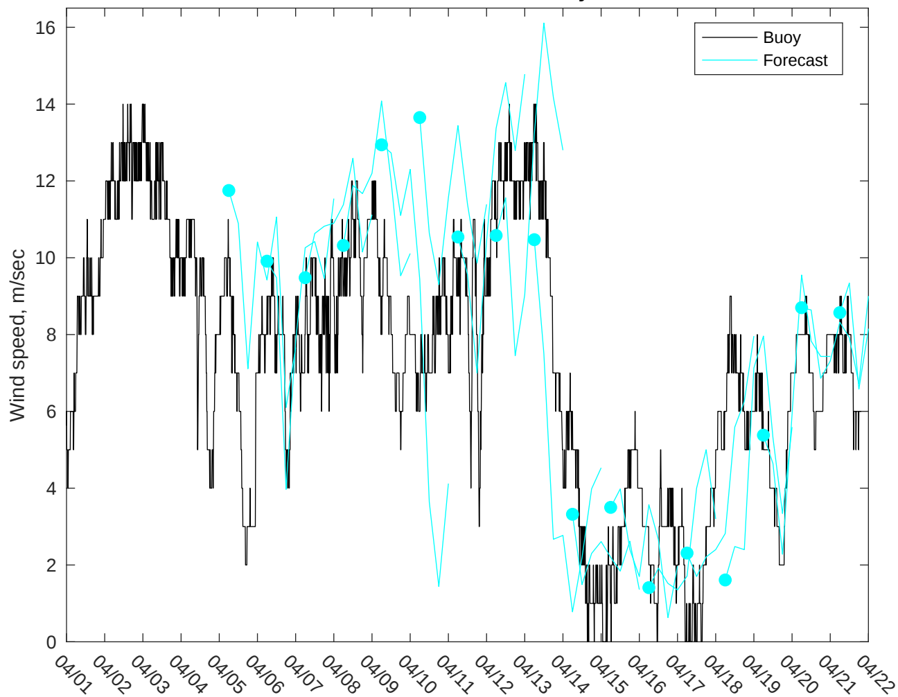
NDBC 46069 vs AUSWAV Winds: 5 to 7 day forecast
