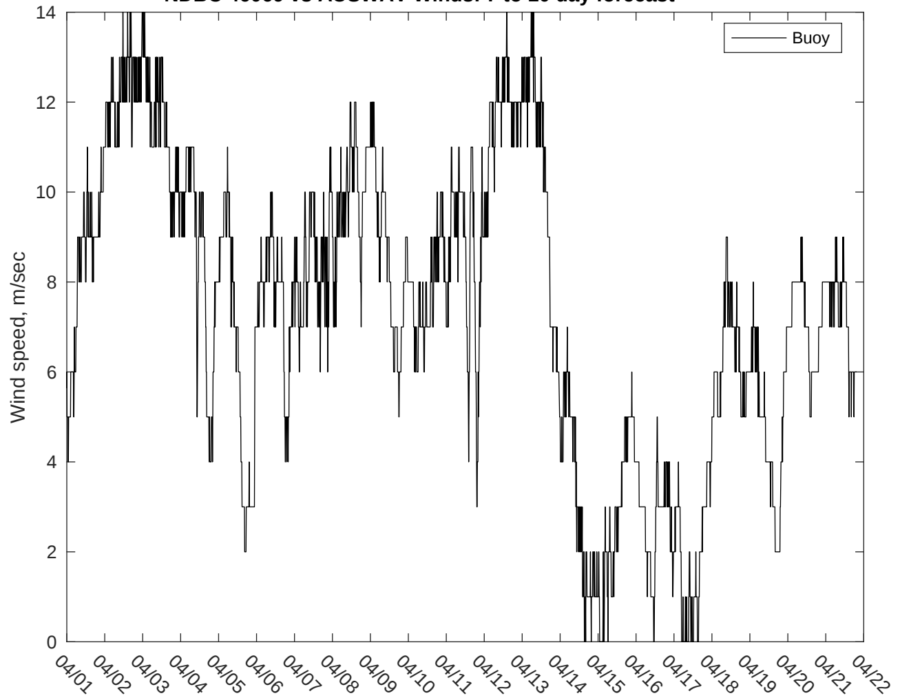
NDBC 46069 vs AUSWAV Winds: 7 to 10 day forecast
