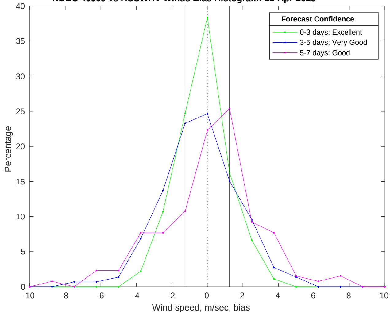
NDBC 46069 vs AUSWAV Winds Bias Histogram: 21-Apr-2025
