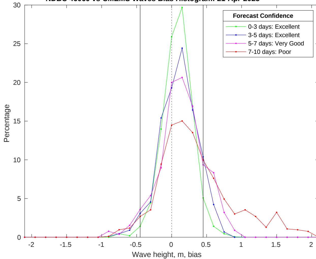
NDBC 46069 vs CMEMS Waves Bias Histogram: 21-Apr-2025
