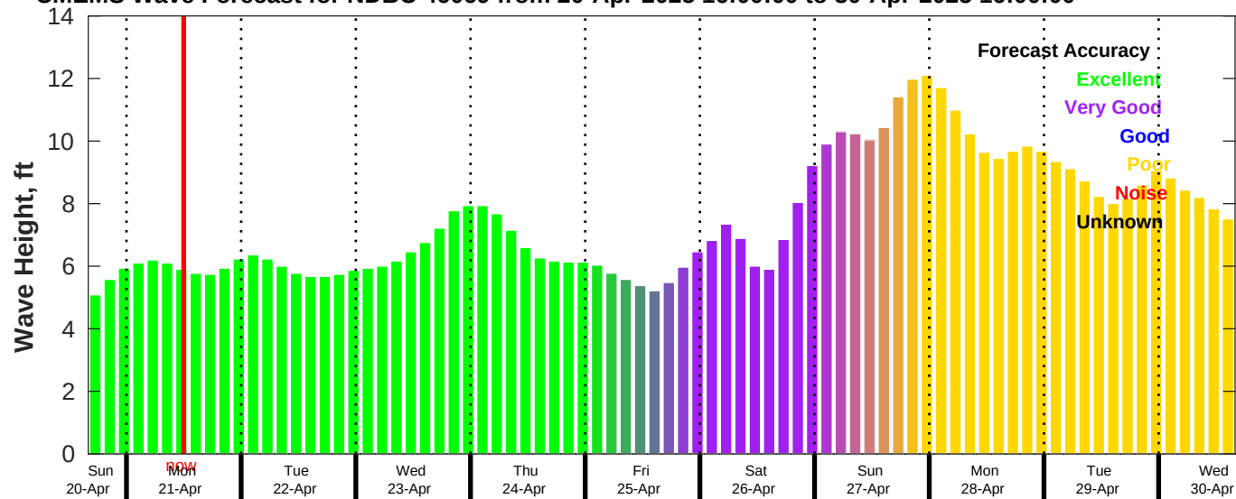
CMEMS Wave Forecast for NDBC 46069 from 20-Apr-2025 16:00:00 to 30-Apr-2025 16:00:00
