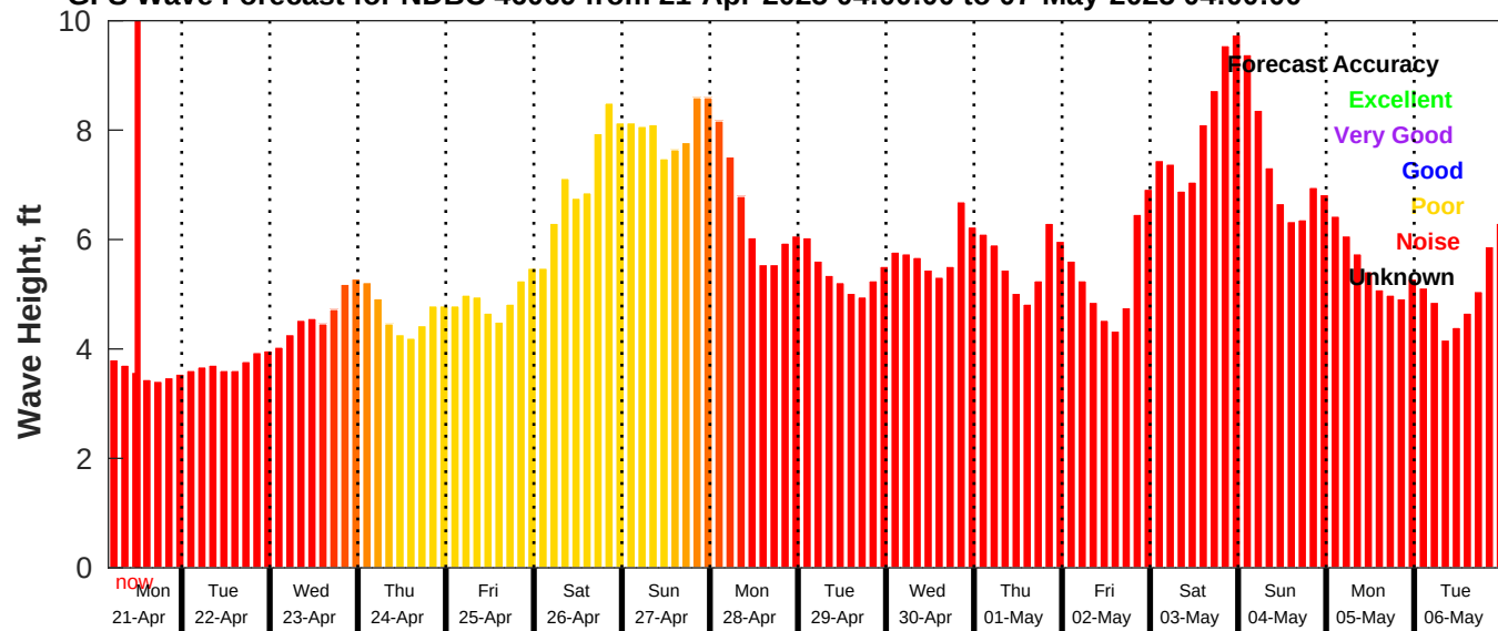
GFS Wave Forecast for NDBC 46069 from 21-Apr-2025 04:00:00 to 07-May-2025 04:00:00
