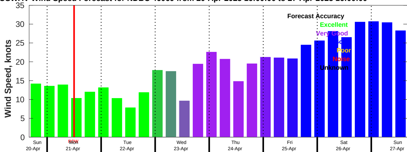
AUSWAV Wind Speed Forecast for NDBC 46069 from 20-Apr-2025 16:00:00 to 27-Apr-2025 16:00:00
