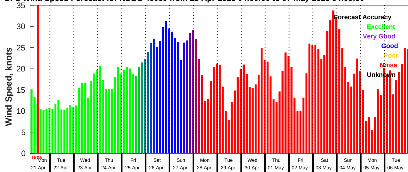
GFS Wind Speed Forecast for NDBC 46069 from 21-Apr-2025 04:00:00 to 07-May-2025 04:00:00
