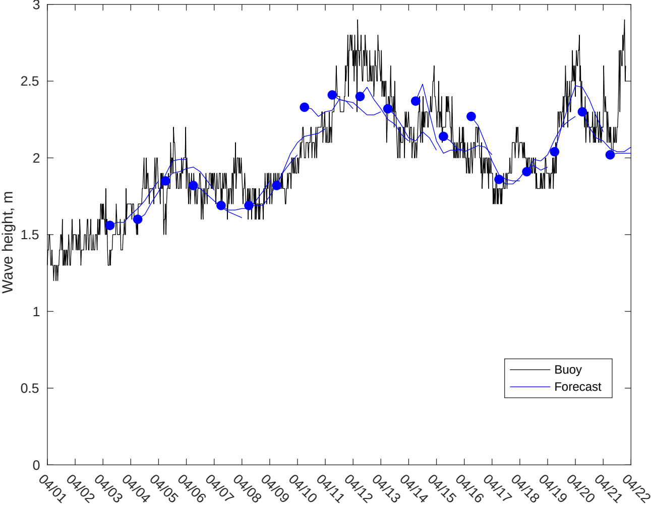
NDBC 51209 vs AUSWAV Waves: 3 to 5 day forecast
