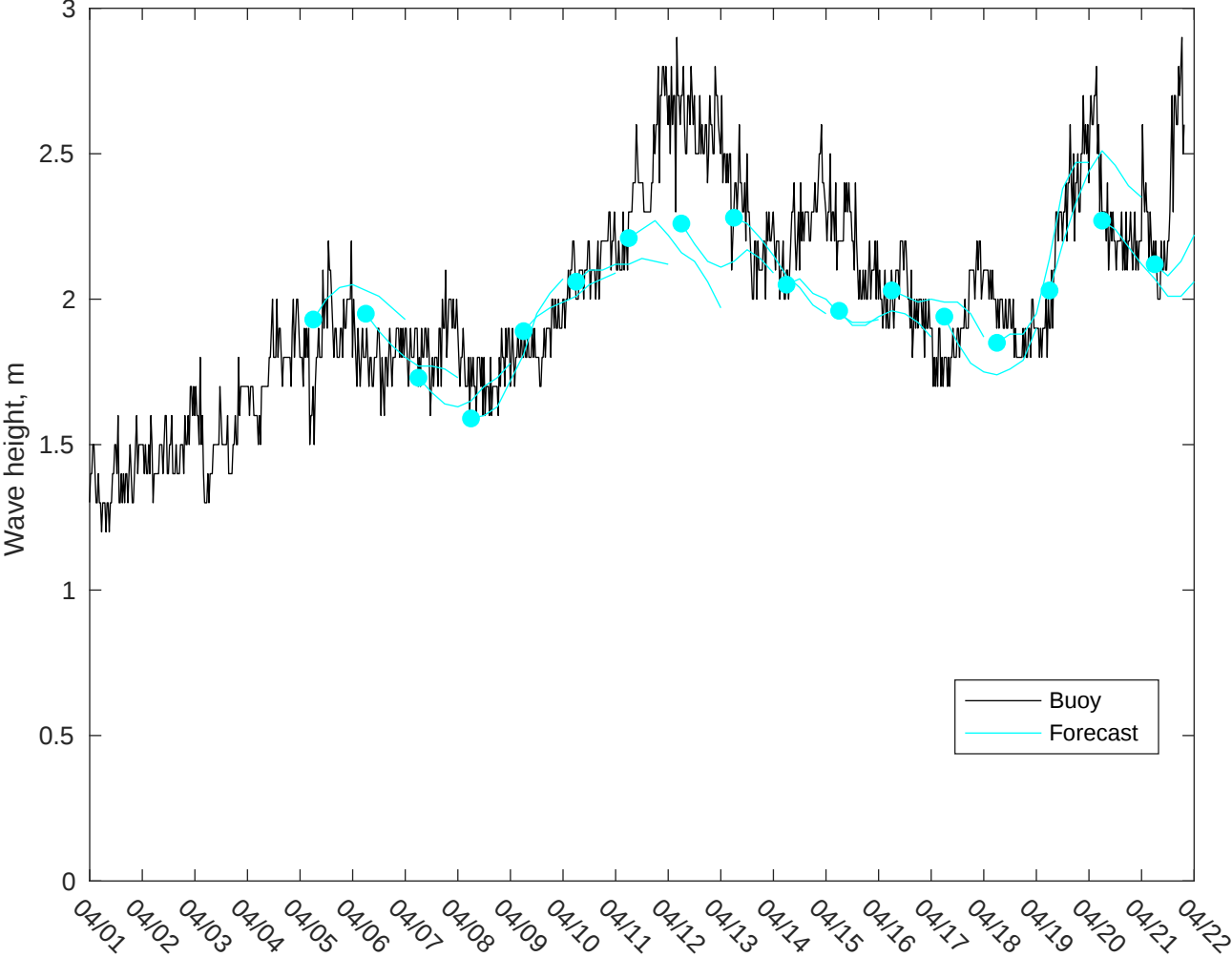
NDBC 51209 vs AUSWAV Waves: 5 to 7 day forecast
