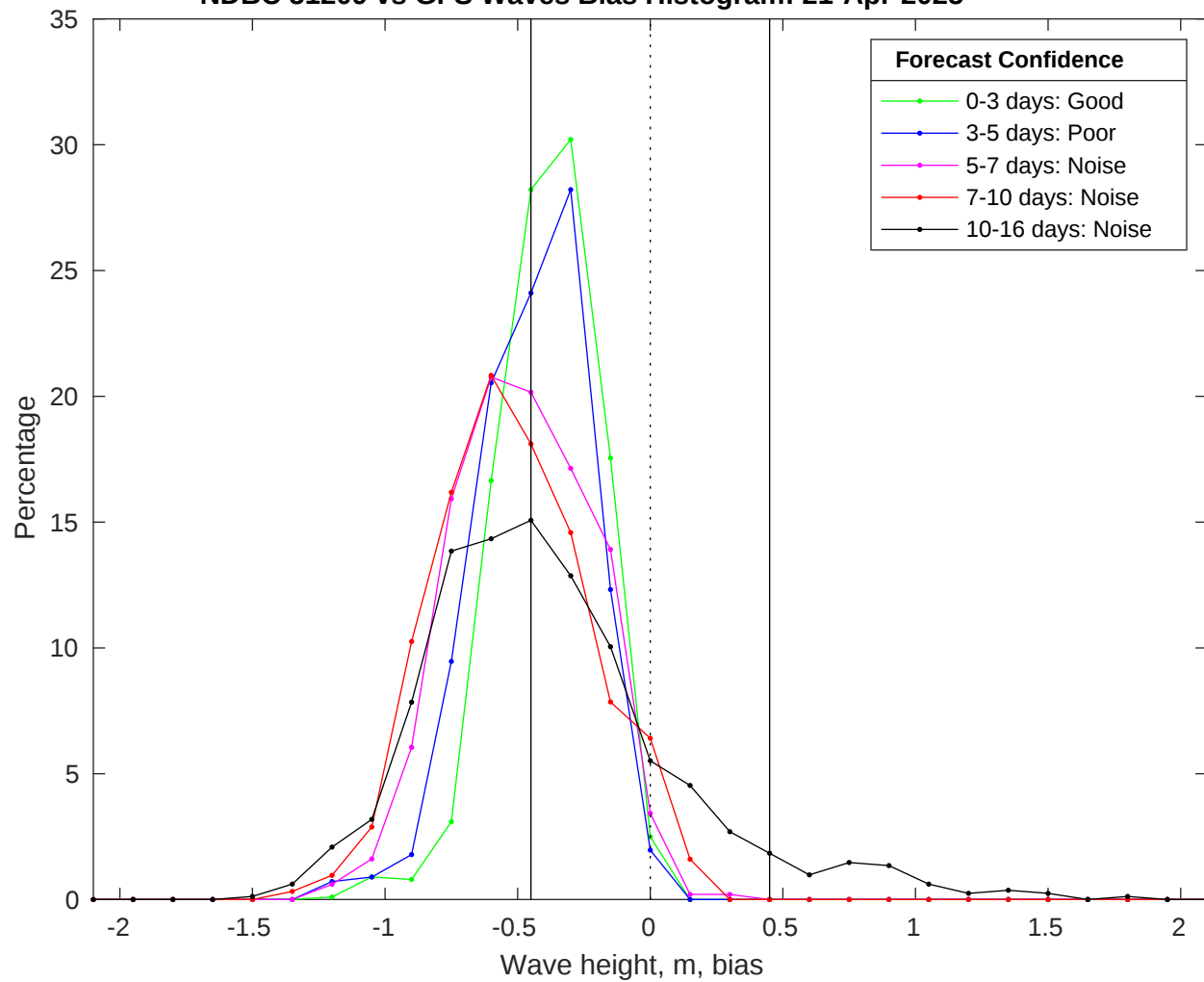
NDBC 51209 vs GFS Waves Bias Histogram: 21-Apr-2025
