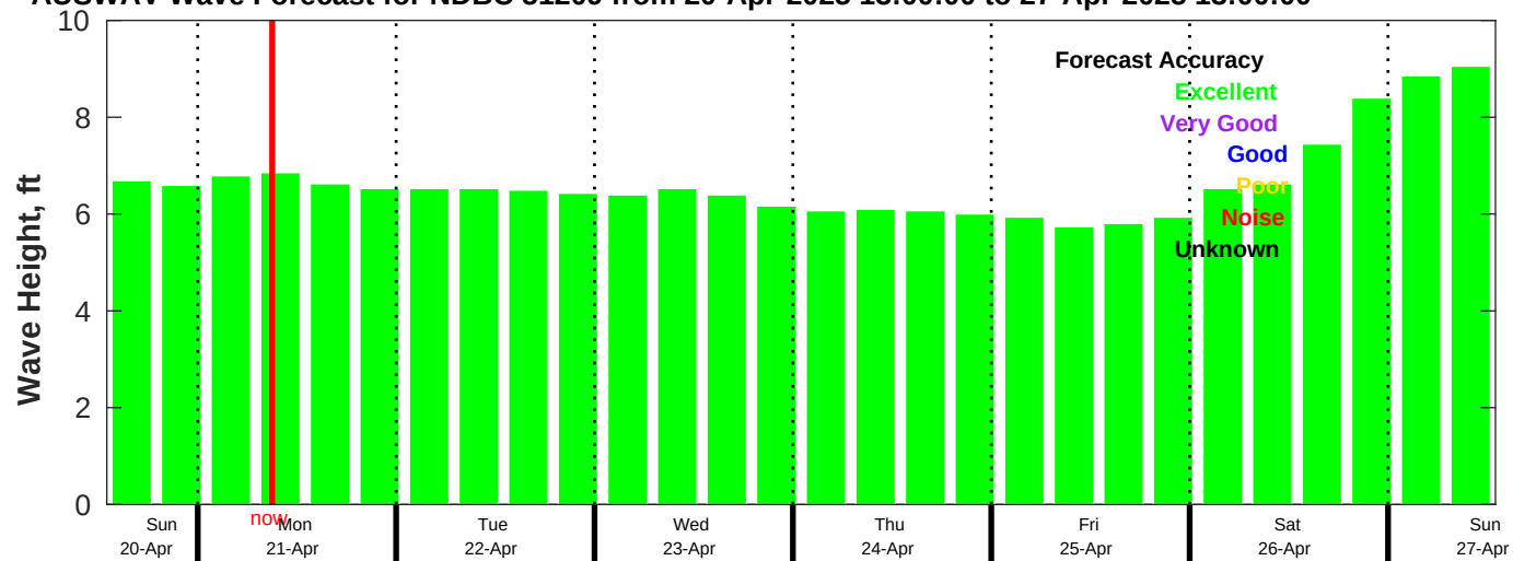
AUSWAV Wave Forecast for NDBC 51209 from 20-Apr-2025 13:00:00 to 27-Apr-2025 13:00:00
