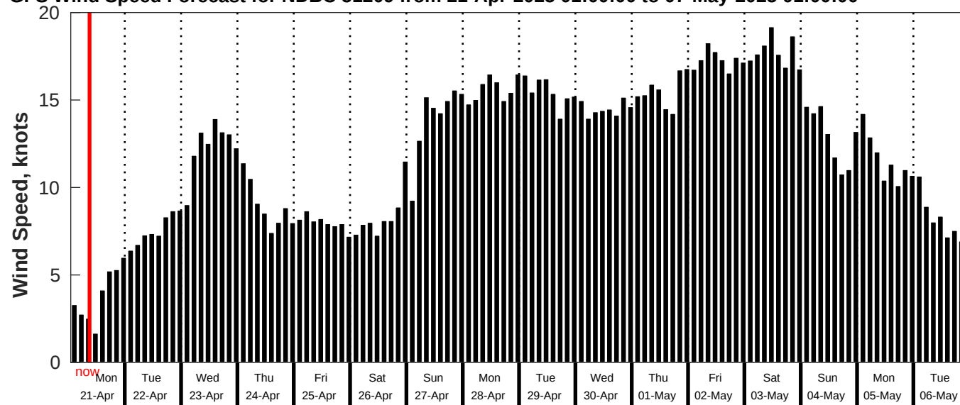
GFS Wind Speed Forecast for NDBC 51209 from 21-Apr-2025 01:00:00 to 07-May-2025 01:00:00
