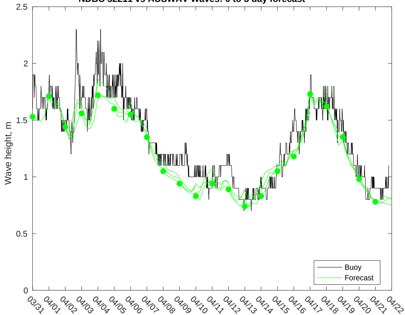
NDBC 52211 vs AUSWAV Waves: 0 to 3 day forecast
