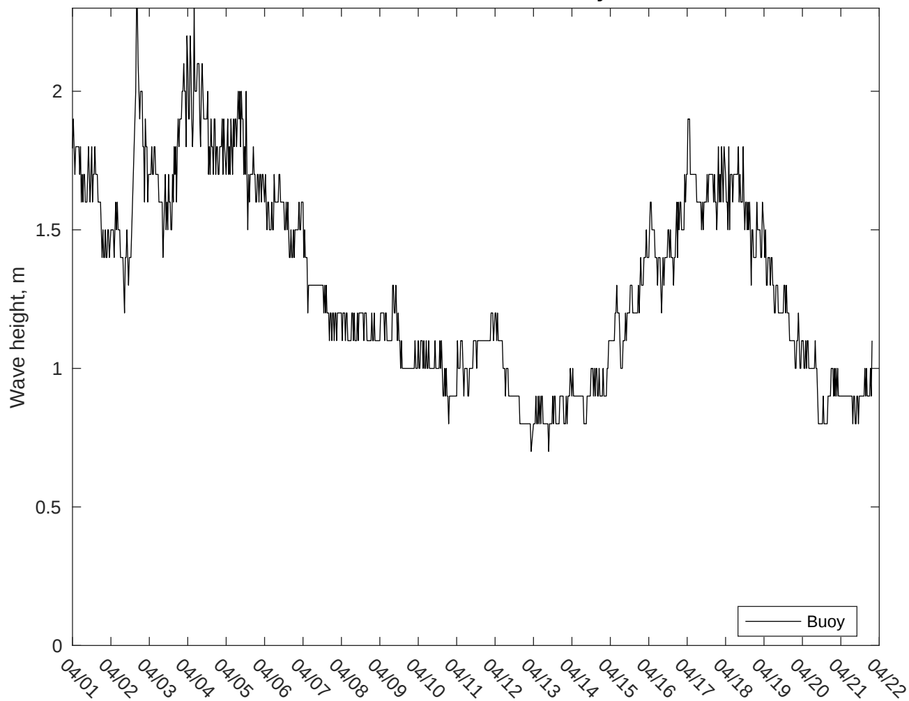
NDBC 52211 vs AUSWAV Waves: 10 to 16 day forecast
