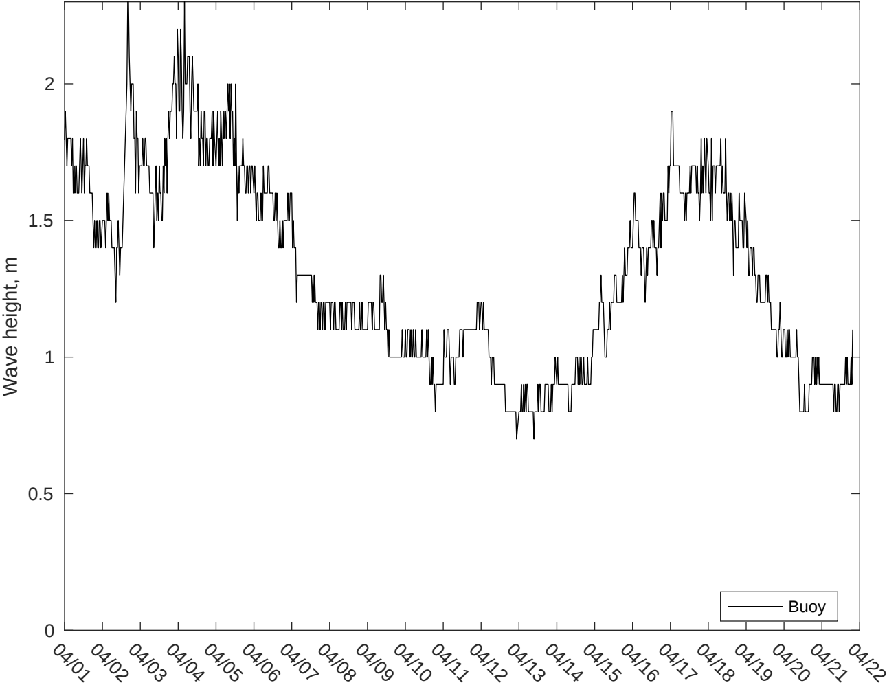
NDBC 52211 vs AUSWAV Waves: 7 to 10 day forecast
