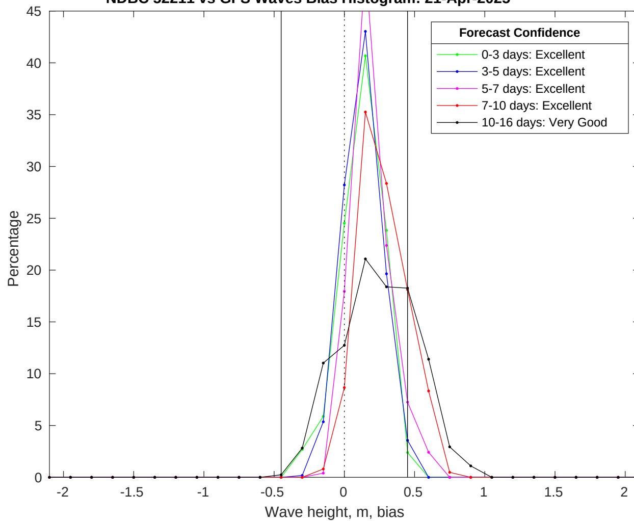
NDBC 52211 vs GFS Waves Bias Histogram: 21-Apr-2025
