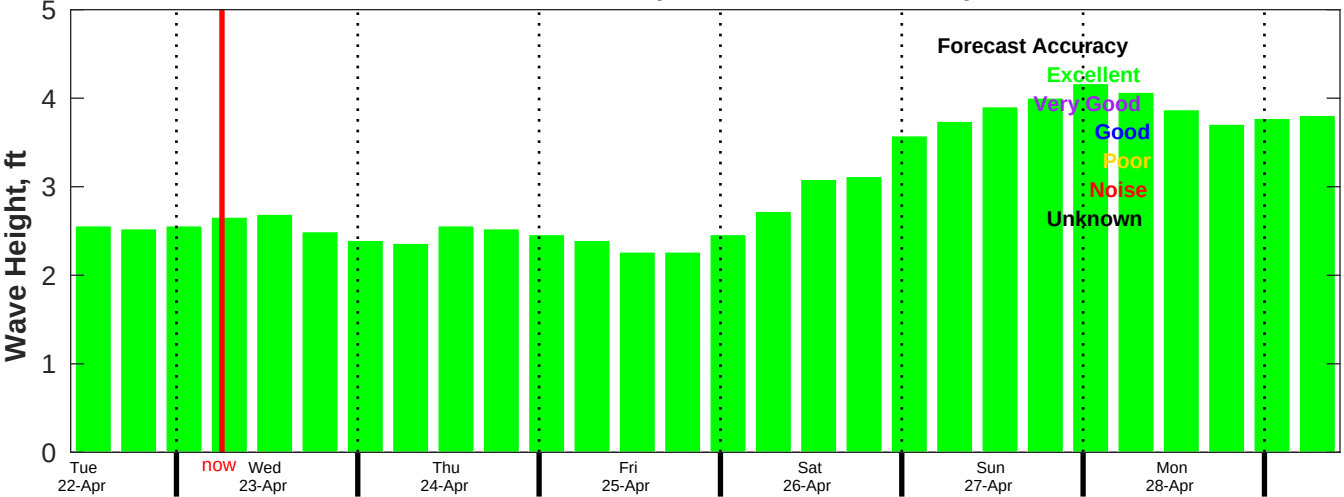
AUSWAV Wave Forecast for NDBC 52211 from 21-Apr-2025 10:00:00 to 28-Apr-2025 10:00:00
