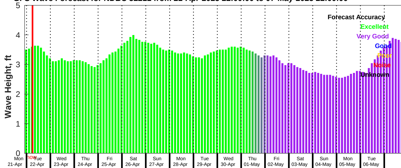
GFS Wave Forecast for NDBC 52211 from 21-Apr-2025 22:00:00 to 07-May-2025 22:00:00
