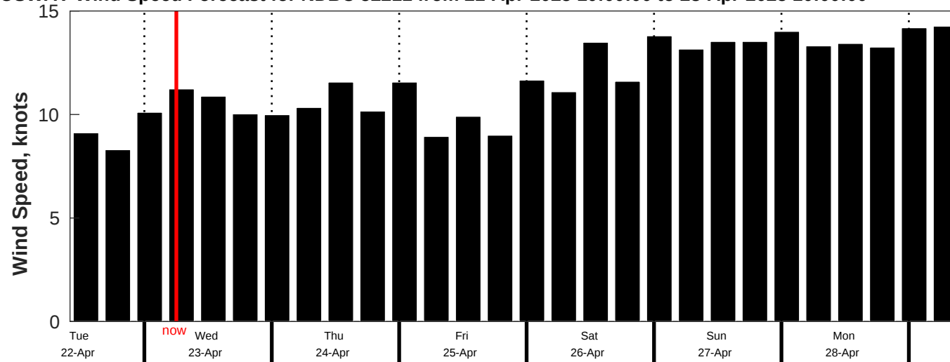
AUSWAV Wind Speed Forecast for NDBC 52211 from 21-Apr-2025 10:00:00 to 28-Apr-2025 10:00:00
