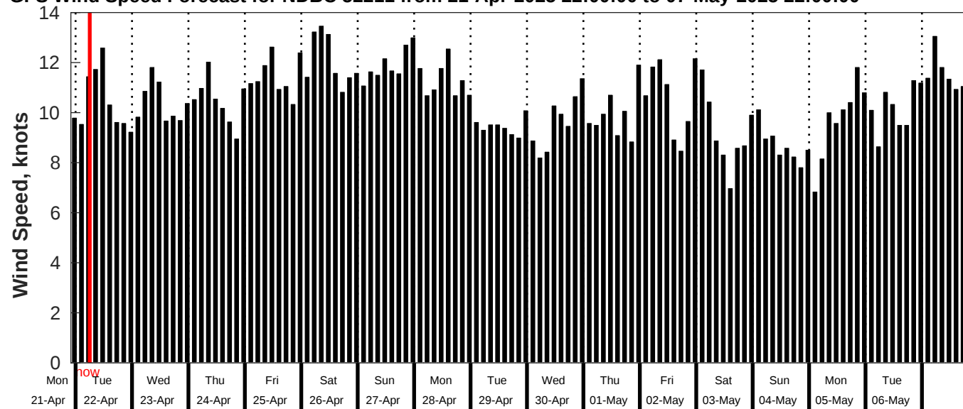
GFS Wind Speed Forecast for NDBC 52211 from 21-Apr-2025 22:00:00 to 07-May-2025 22:00:00
