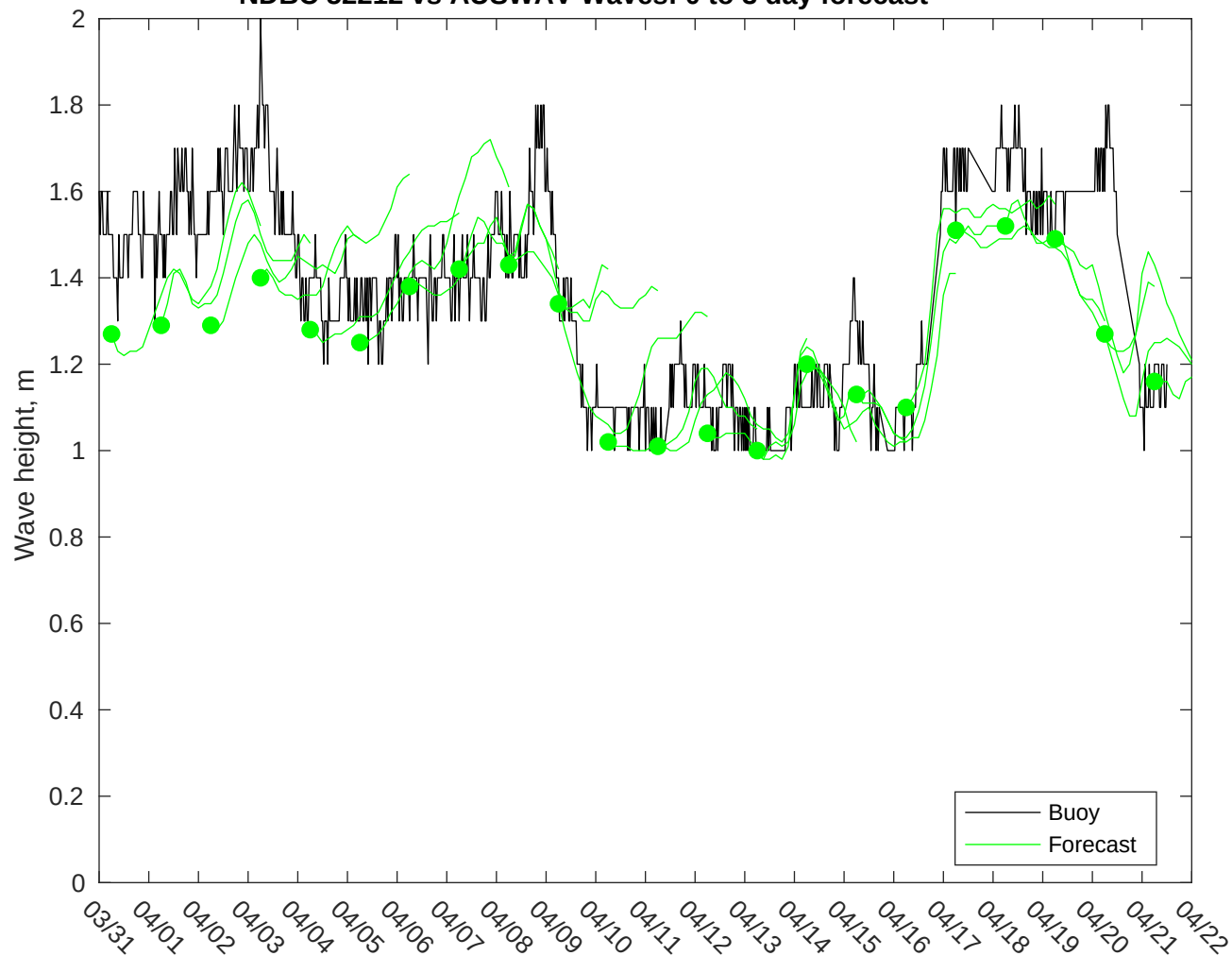
NDBC 52212 vs AUSWAV Waves: 0 to 3 day forecast
