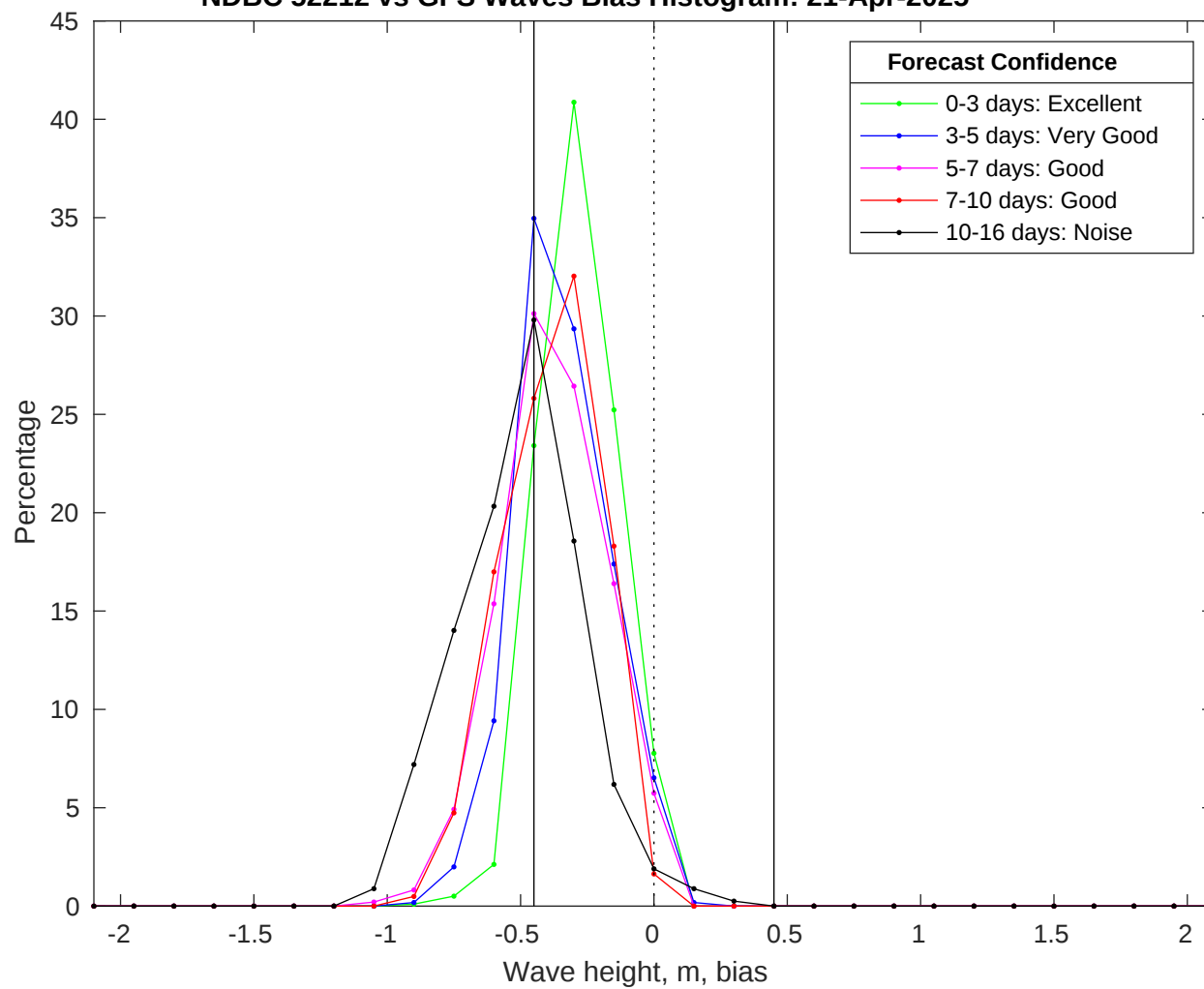
NDBC 52212 vs GFS Waves Bias Histogram: 21-Apr-2025
