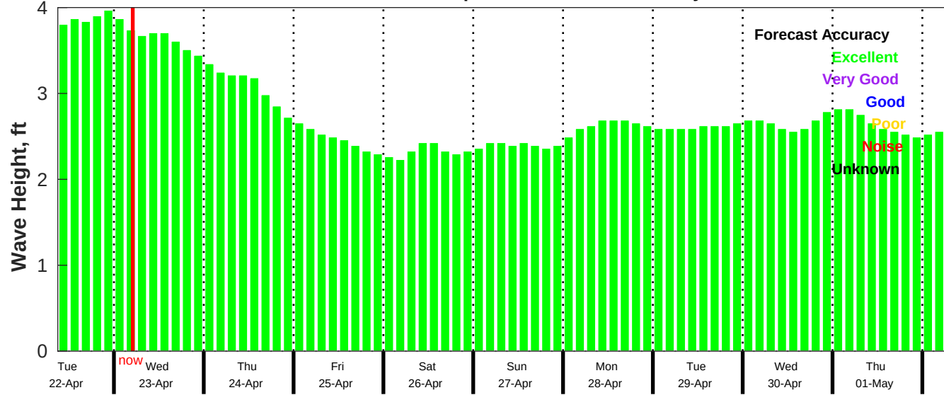
CMEMS Wave Forecast for NDBC 52212 from 21-Apr-2025 09:00:00 to 01-May-2025 09:00:00
