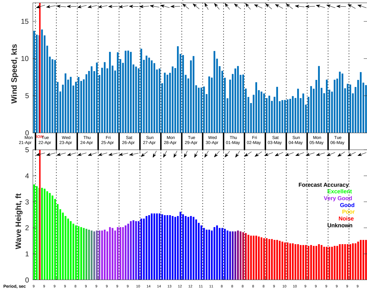
Wind & Wave Forecast for NDBC 52212 from 21-Apr-2025 21:00:00 to 07-May-2025 21:00:00
