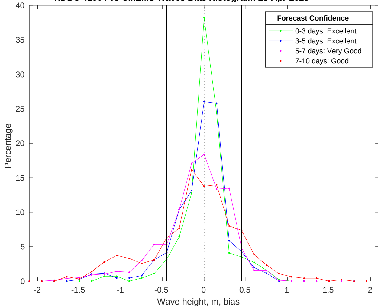
NDBC 41004 vs CMEMS Waves Bias Histogram: 23-Apr-2025
