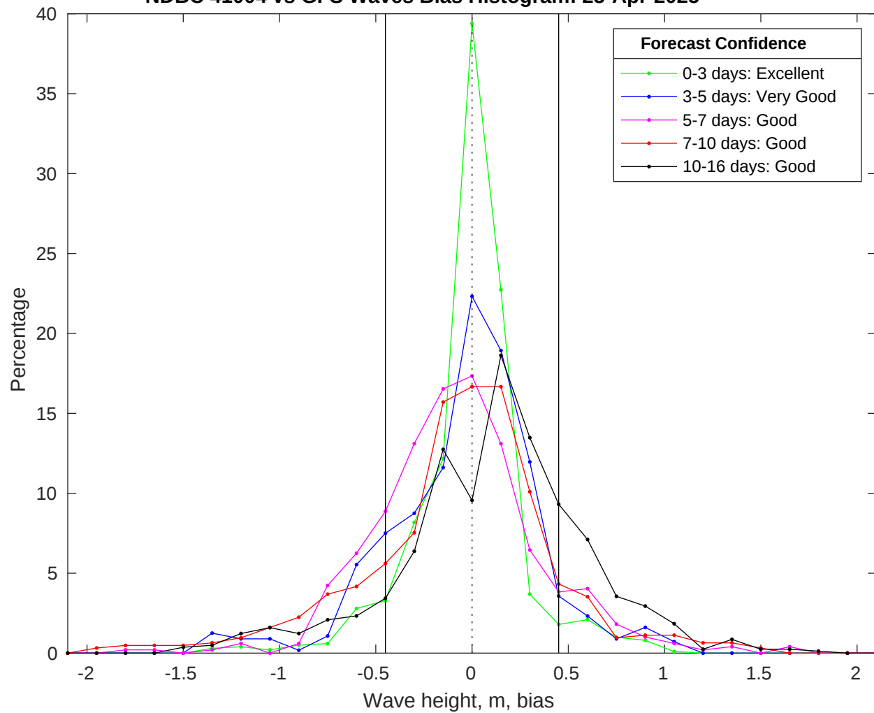
NDBC 41004 vs GFS Waves Bias Histogram: 23-Apr-2025
