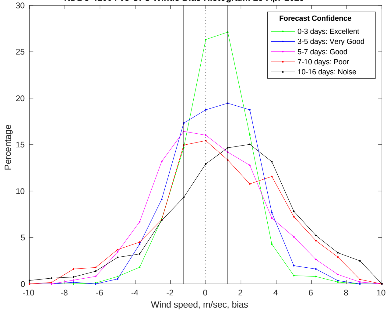
NDBC 41004 vs GFS Winds Bias Histogram: 23-Apr-2025
