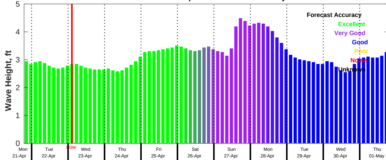
CMEMS Wave Forecast for NDBC 41004 from 21-Apr-2025 19:00:00 to 01-May-2025 19:00:00
