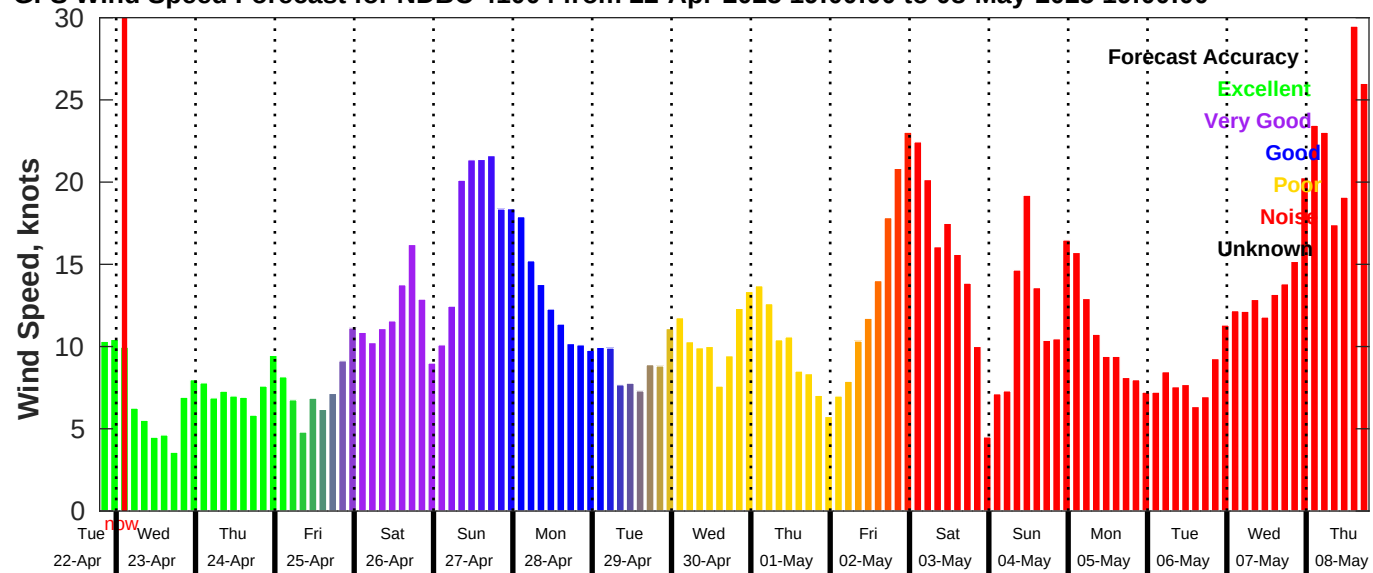
GFS Wind Speed Forecast for NDBC 41004 from 22-Apr-2025 19:00:00 to 08-May-2025 19:00:00
