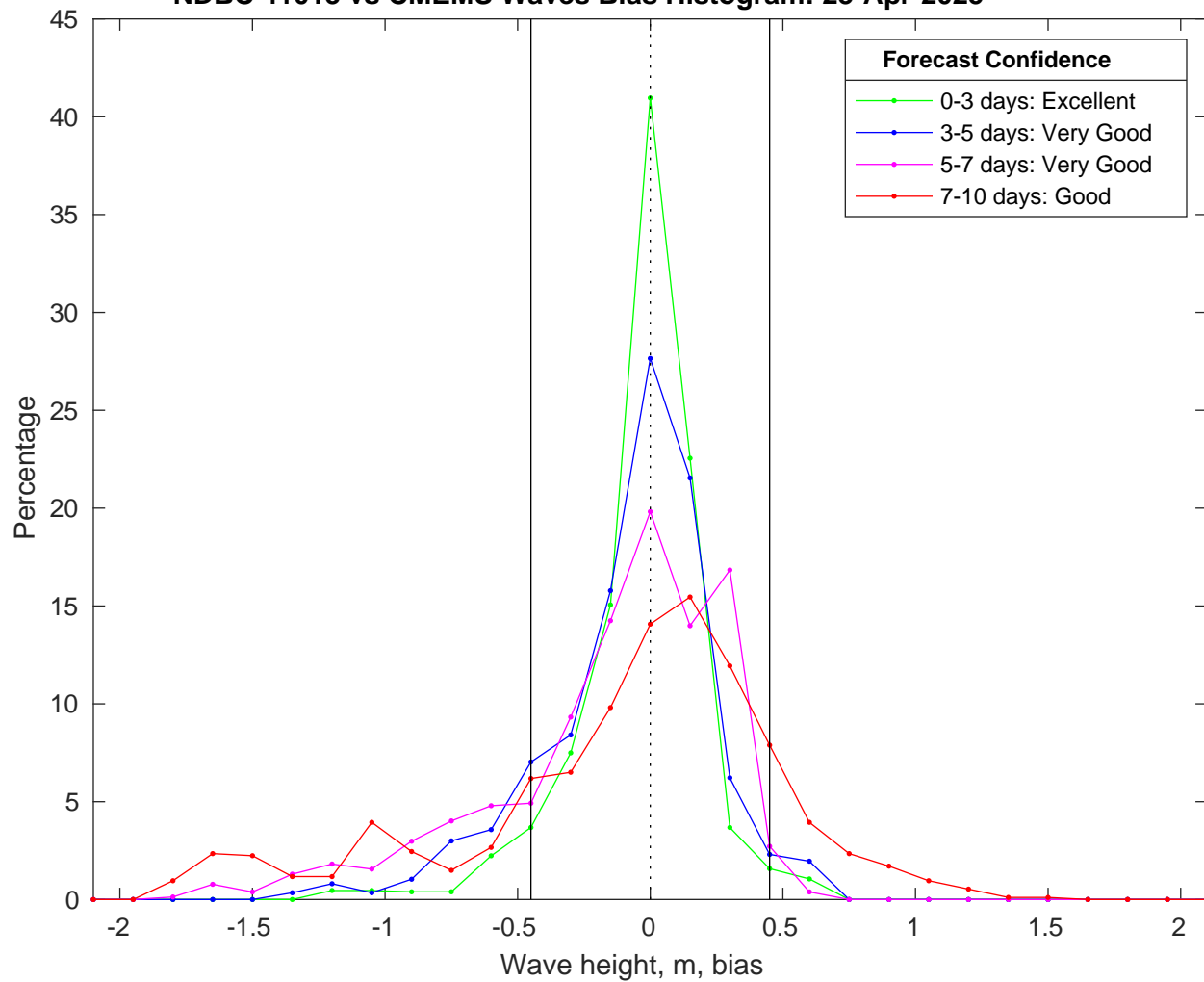
NDBC 41013 vs CMEMS Waves Bias Histogram: 23-Apr-2025
