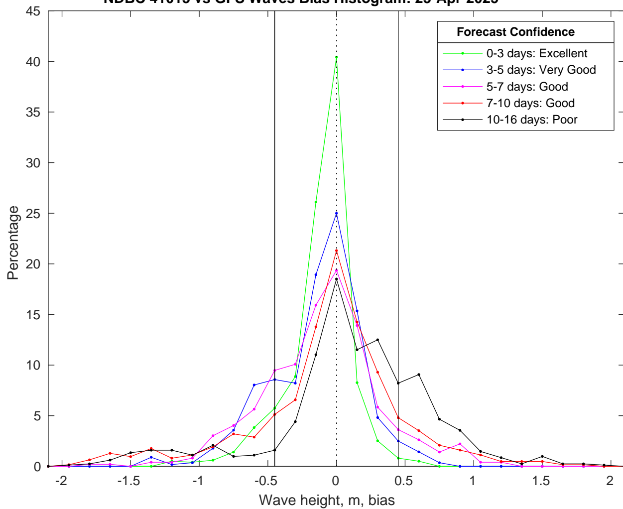
NDBC 41013 vs GFS Waves Bias Histogram: 23-Apr-2025
