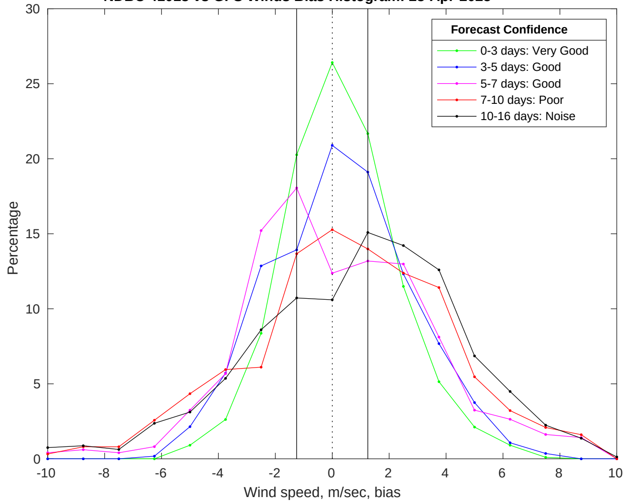
NDBC 41013 vs GFS Winds Bias Histogram: 23-Apr-2025
