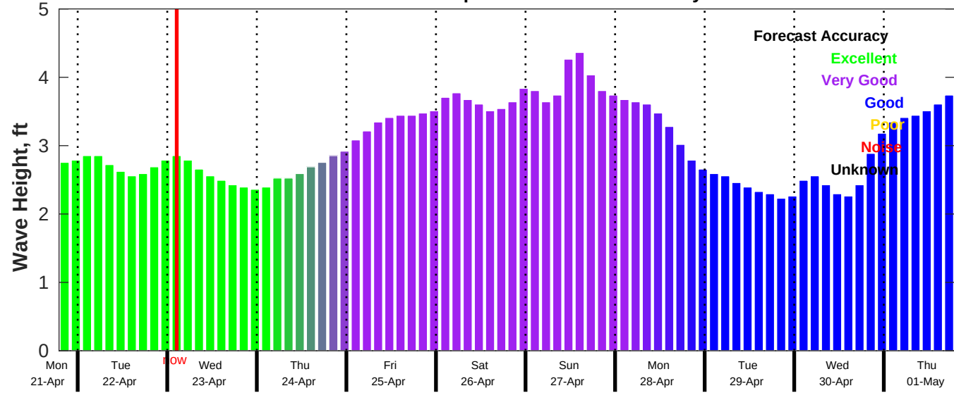
CMEMS Wave Forecast for NDBC 41013 from 21-Apr-2025 19:00:00 to 01-May-2025 19:00:00
