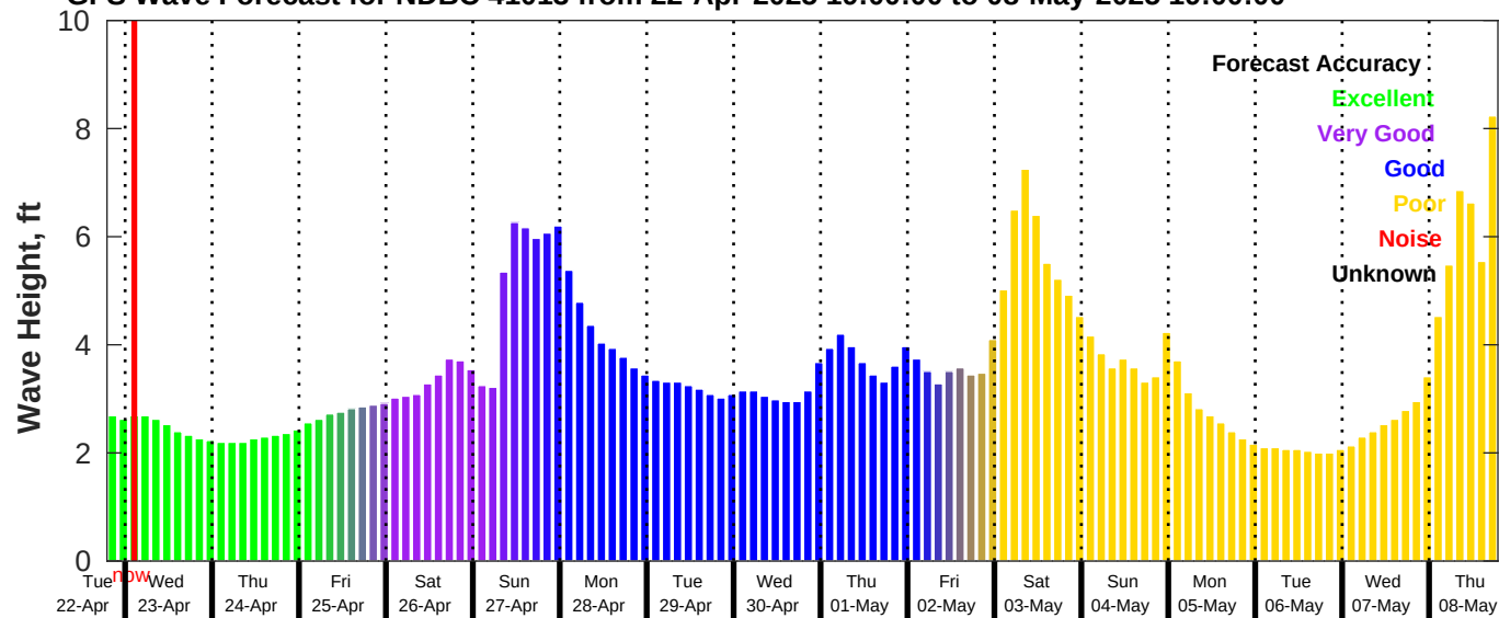
GFS Wave Forecast for NDBC 41013 from 22-Apr-2025 19:00:00 to 08-May-2025 19:00:00
