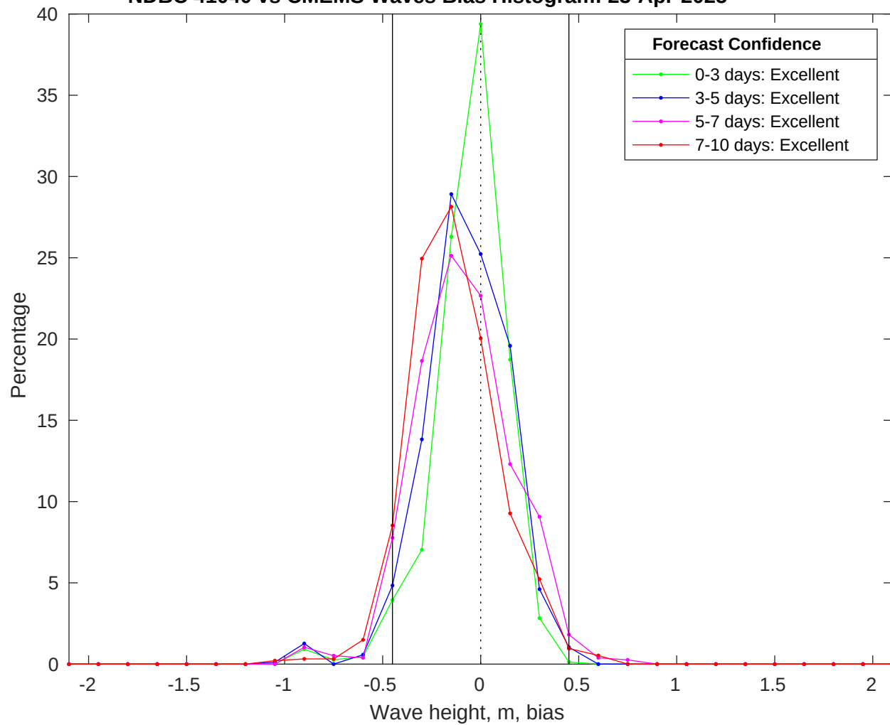
NDBC 41040 vs CMEMS Waves Bias Histogram: 23-Apr-2025
