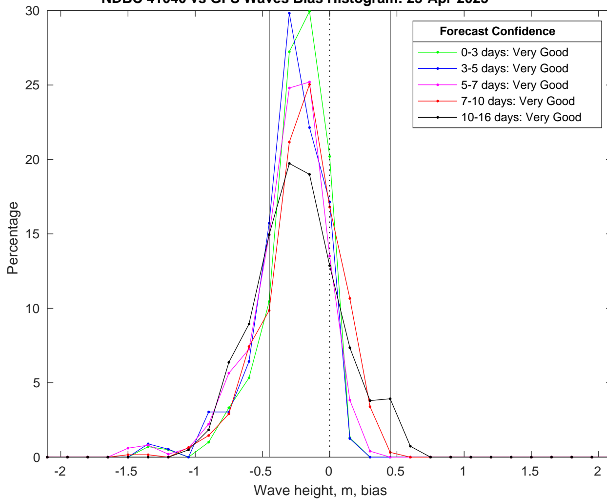
NDBC 41040 vs GFS Waves Bias Histogram: 23-Apr-2025
