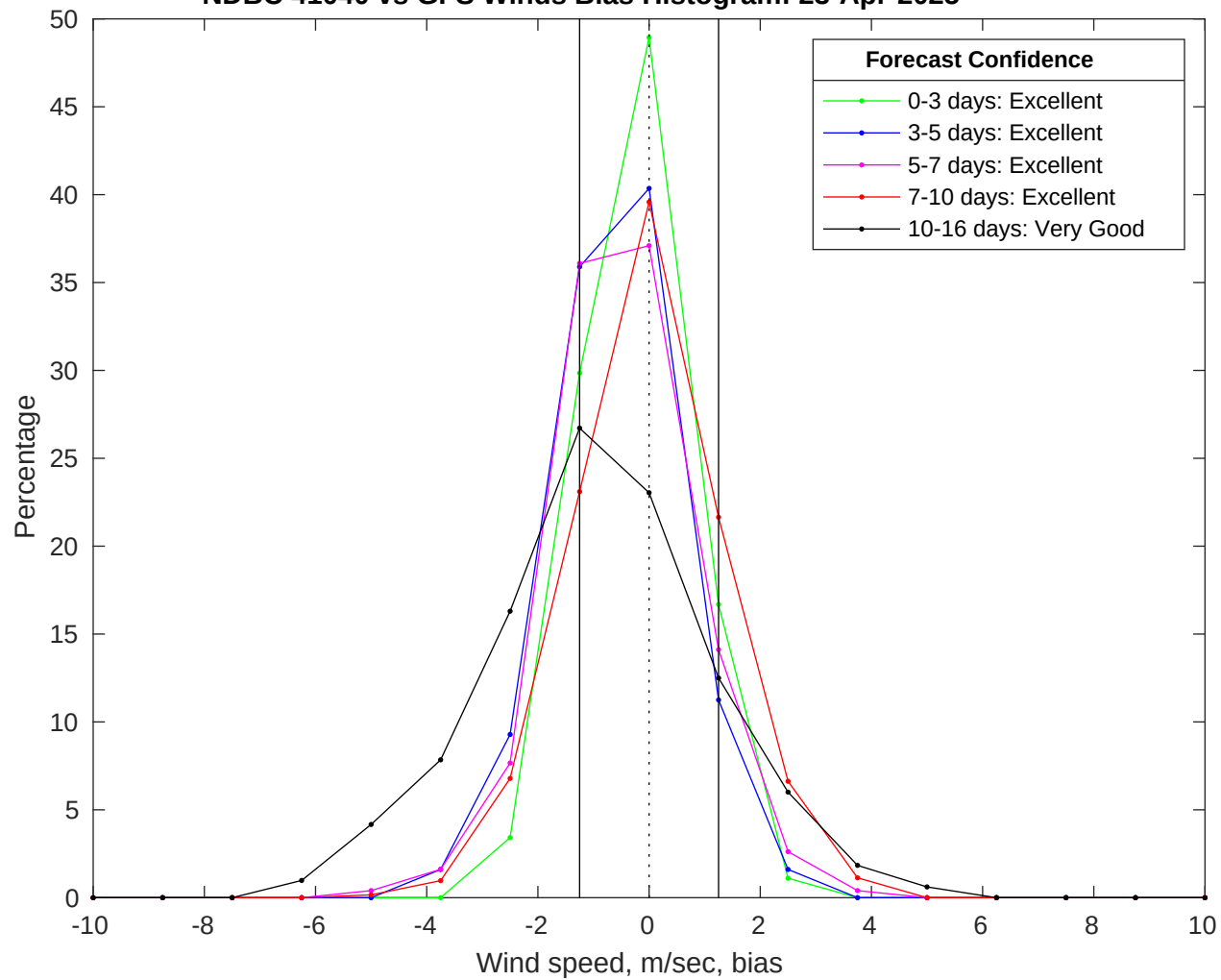
NDBC 41040 vs GFS Winds Bias Histogram: 23-Apr-2025
