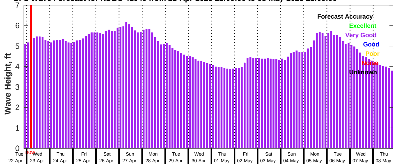
GFS Wave Forecast for NDBC 41040 from 22-Apr-2025 21:00:00 to 08-May-2025 21:00:00
