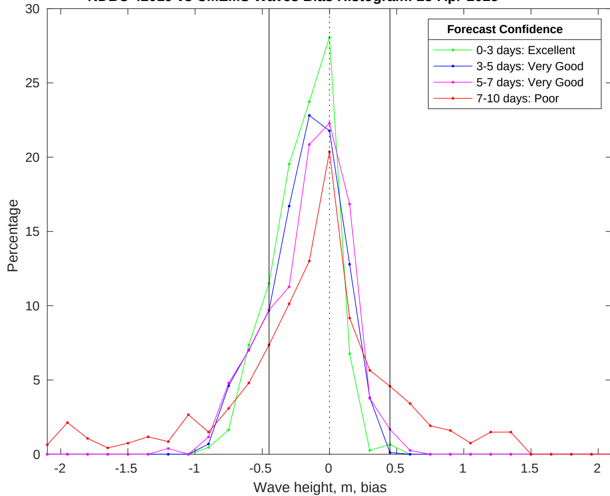
NDBC 42019 vs CMEMS Waves Bias Histogram: 23-Apr-2025
