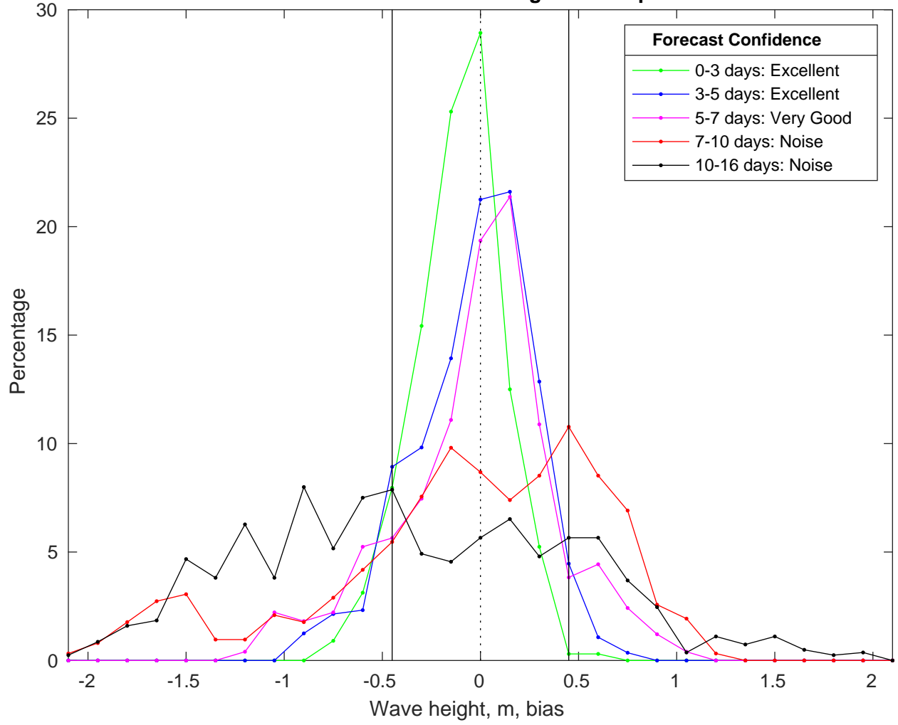
NDBC 42019 vs GFS Waves Bias Histogram: 23-Apr-2025
