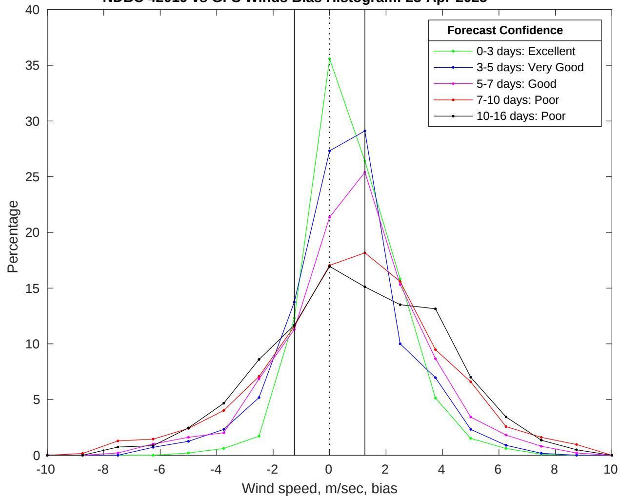
NDBC 42019 vs GFS Winds Bias Histogram: 23-Apr-2025
