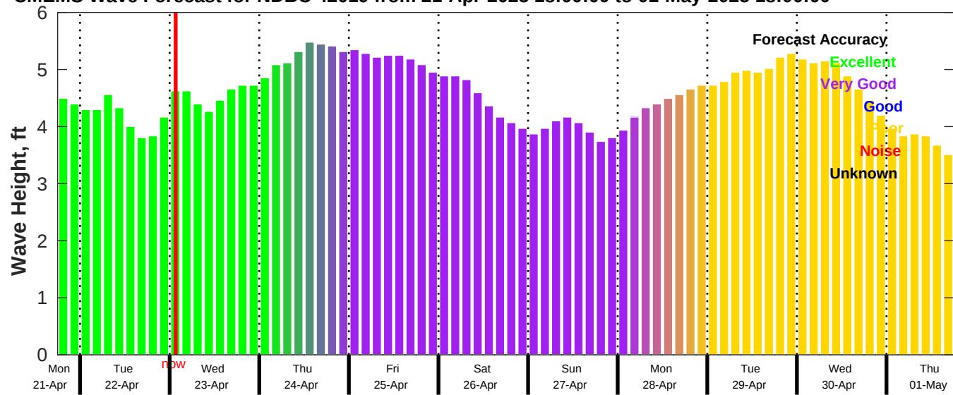
CMEMS Wave Forecast for NDBC 42019 from 21-Apr-2025 18:00:00 to 01-May-2025 18:00:00
