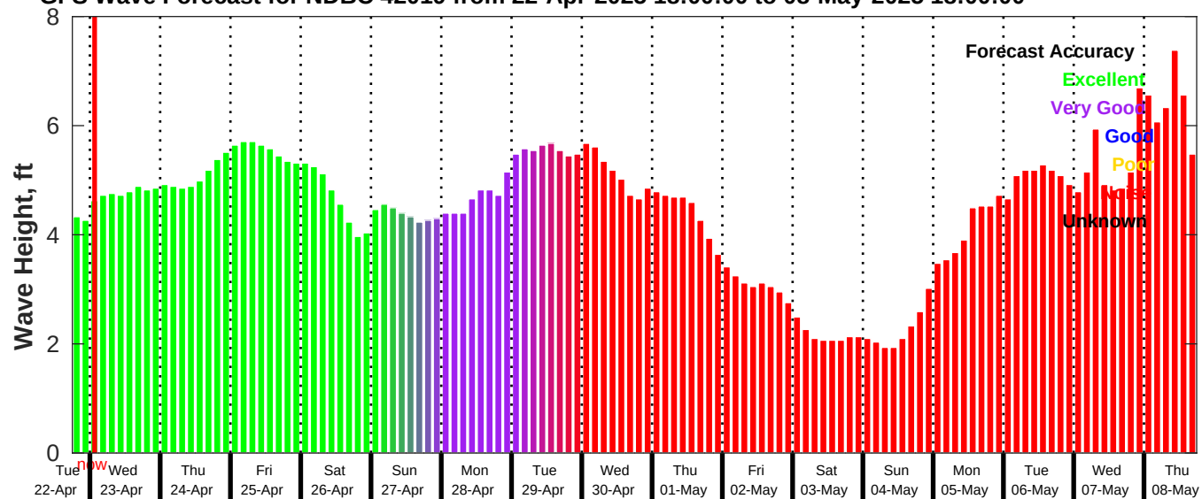
GFS Wave Forecast for NDBC 42019 from 22-Apr-2025 18:00:00 to 08-May-2025 18:00:00
