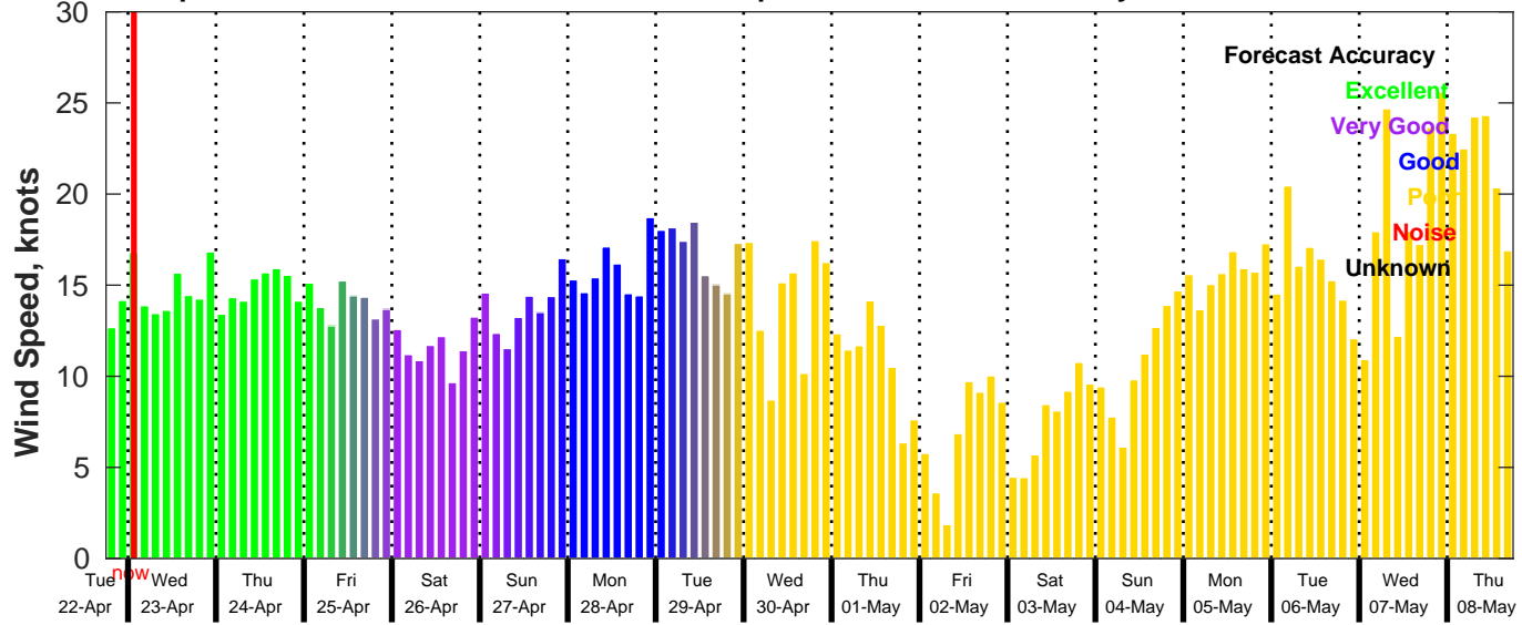
GFS Wind Speed Forecast for NDBC 42019 from 22-Apr-2025 18:00:00 to 08-May-2025 18:00:00
