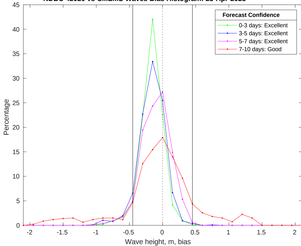
NDBC 42020 vs CMEMS Waves Bias Histogram: 23-Apr-2025
