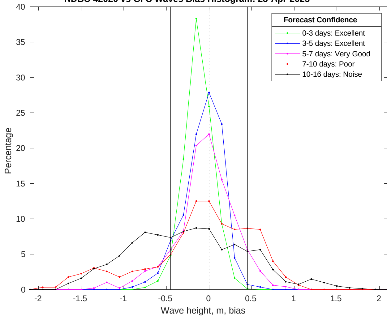
NDBC 42020 vs GFS Waves Bias Histogram: 23-Apr-2025
