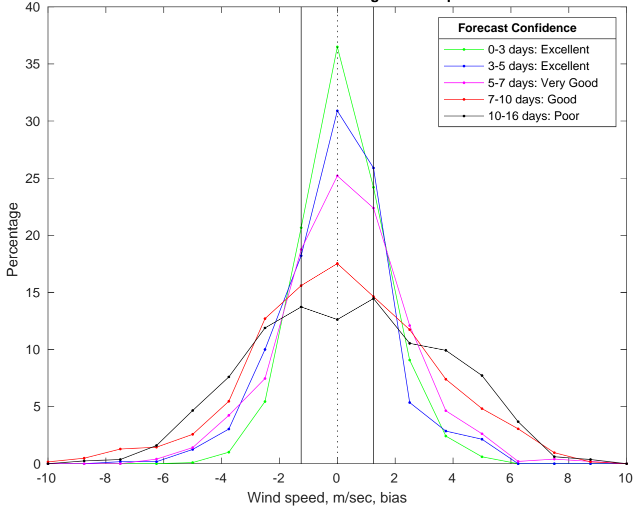
NDBC 42020 vs GFS Winds Bias Histogram: 23-Apr-2025
