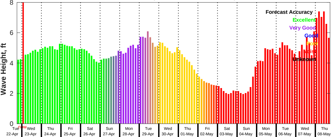
GFS Wave Forecast for NDBC 42020 from 22-Apr-2025 18:00:00 to 08-May-2025 18:00:00
