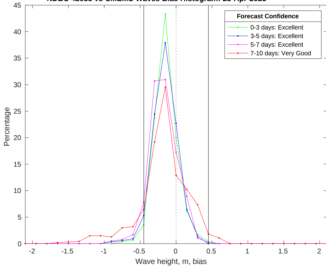
NDBC 42035 vs CMEMS Waves Bias Histogram: 23-Apr-2025
